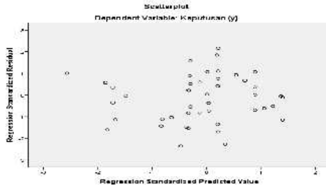
Gambar 3 Hasil Scatterplot
