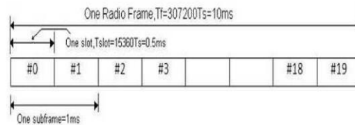
Figure 2. LTE-Frame Structure, FDD
