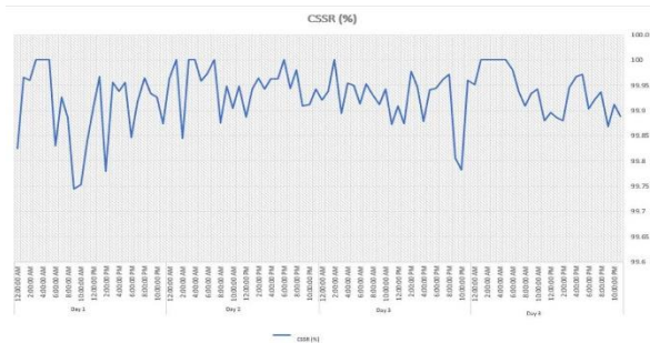
Figure 11. CSSR in 15 MHz Bandwidth.
