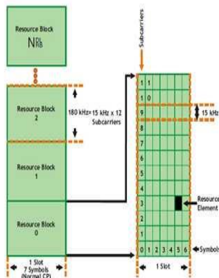
Figure 4. LTE DL PRB allocation over the time and frequency domain
