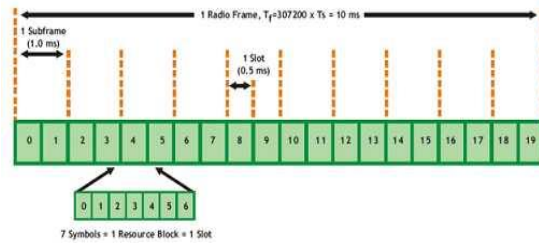
Figure 5. LTE Sub-frame with 20 MHz Bandwidth
