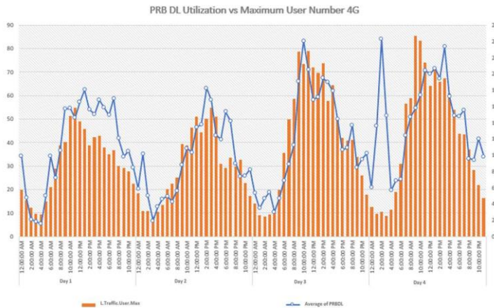
Figure 9. PRB Downlink and Number of User in 15 MHz
