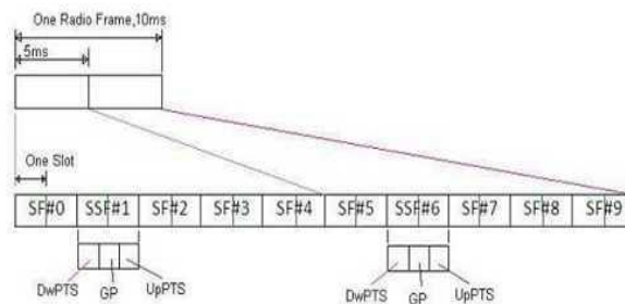
Figure 3. LTE Frame Structure, TDD
