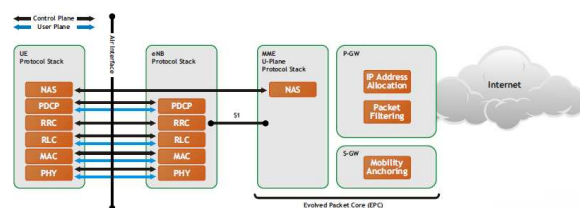
Figure 6. Air Interface in 4G-LTE Network
