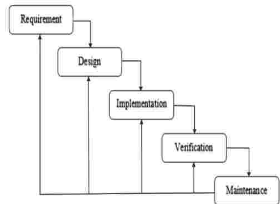
Gambar 1: Metode Waterfall
