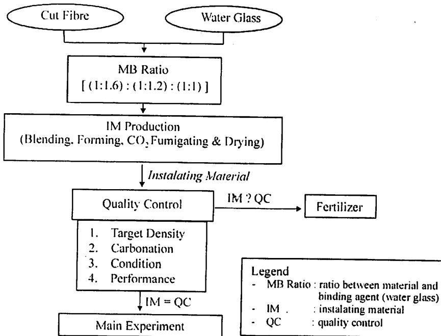
Figure 2. Optimization process of insulation material production
