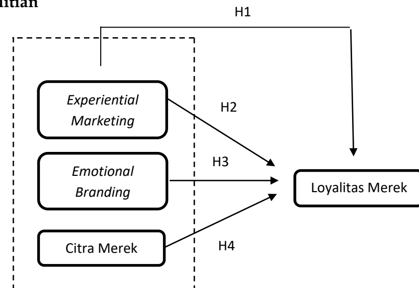
Gambar 1. Model Penelitian
