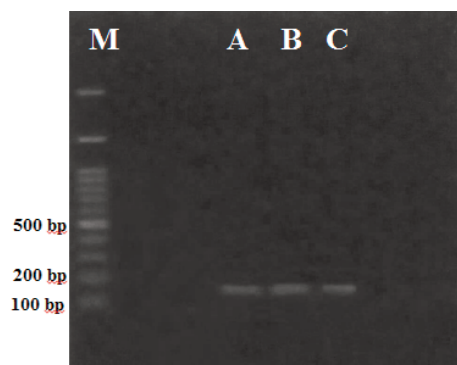
Figure 1. Visualization of PCR products of mosaic leaves and stunting samples; the DNA bands were amplified by CMV 111 specific primer (111 bp); lanes A–C = infected pepper samples; lane M = 100 bp DNA ladder
