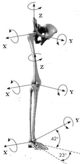
Figure 1. The degrees of freedom of the lower limb
