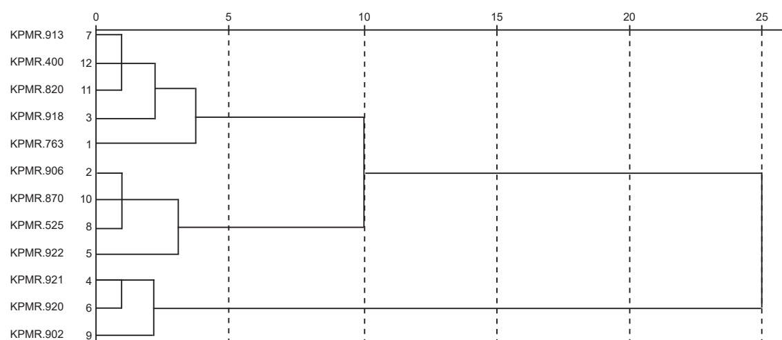
Dendrogram Using Average Linkage (Between Groups) (Rescale Distance Cluster Combine)
