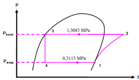
Gambar 4.4. Diagram p-h siklus ideal
