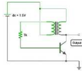
Gambar 8. Rangkaian inverter DC to AC satu transistor
