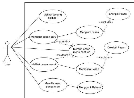
Gambar 6. Use case diagram aplikasi Crypto Messenger
