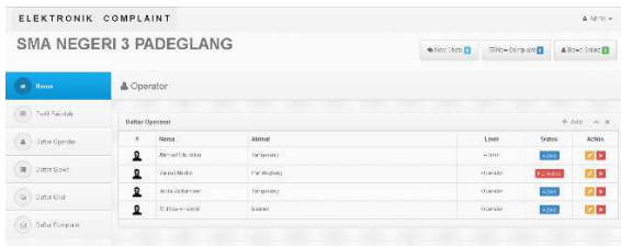
Gambar 4.4. Halaman Operator
