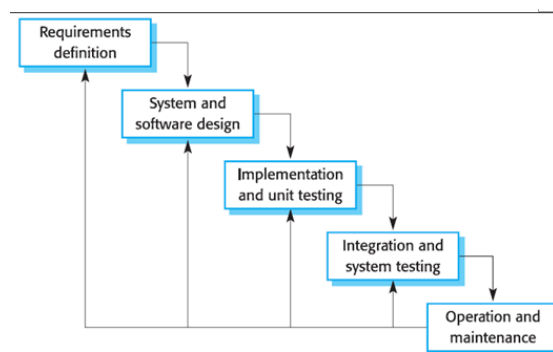
Gambar 2.1. Model Waterfall
