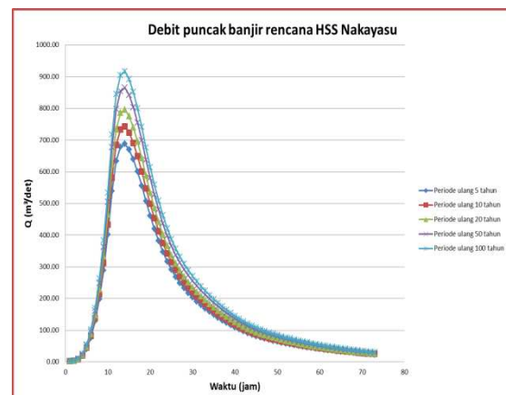
Gambar 1 Debit Puncak Banjir Rencana HSS Nakayasu
