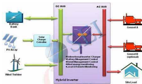
Gambar 2.9 Sistem PLTH Surya, Angin, Diesel
