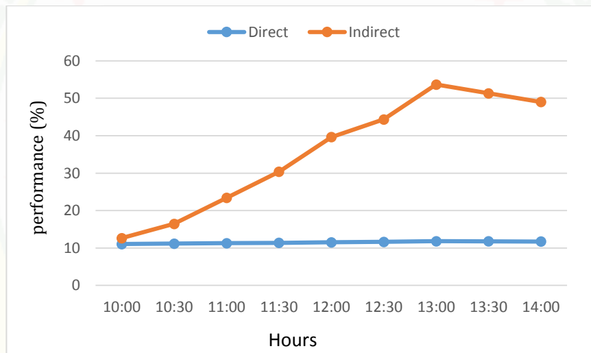
Figure 5. Performance of both dryers
