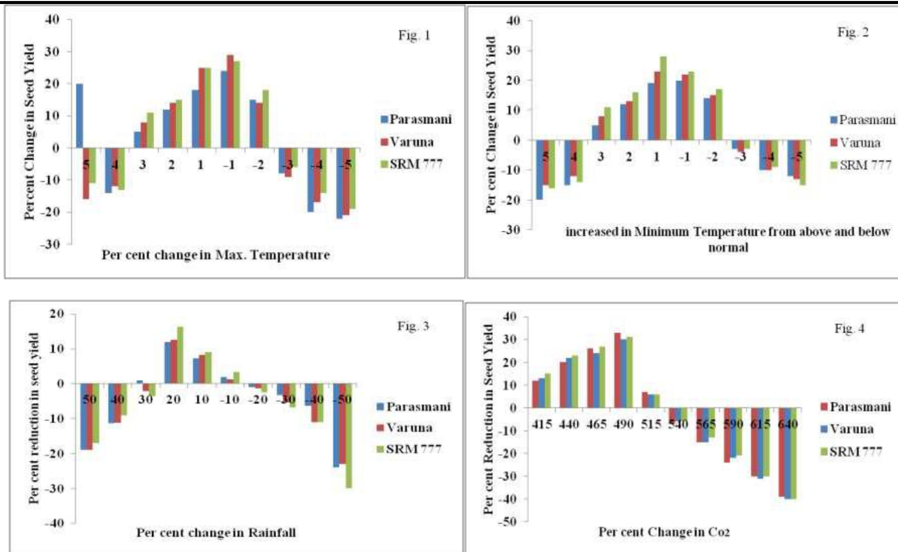
Fig.1: Depicting the InfoCrop simulation results of impact of change in (1) maximum temperature ( T_{max} ) (2) minimum temperature ( T_{min} ) (3) seasonal rainfall and (4) elevation in CO_2 concentration on the seed yield of all three varieties of mustard during the Rabi- 2016-2017.
