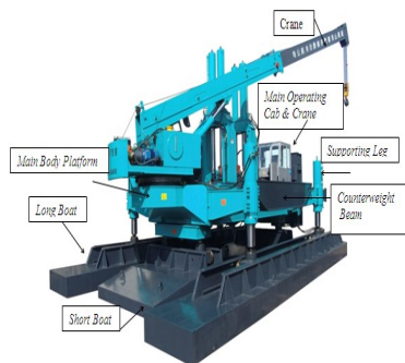
Gambar 1. Hydraulic static pile driver
