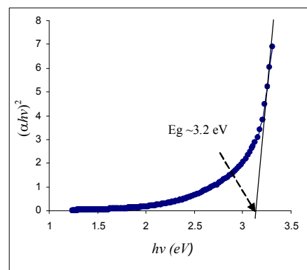
Gambar 5. Plot (\alpha h\nu)^2 terhadap energi foton absorpsi ( h\nu )
