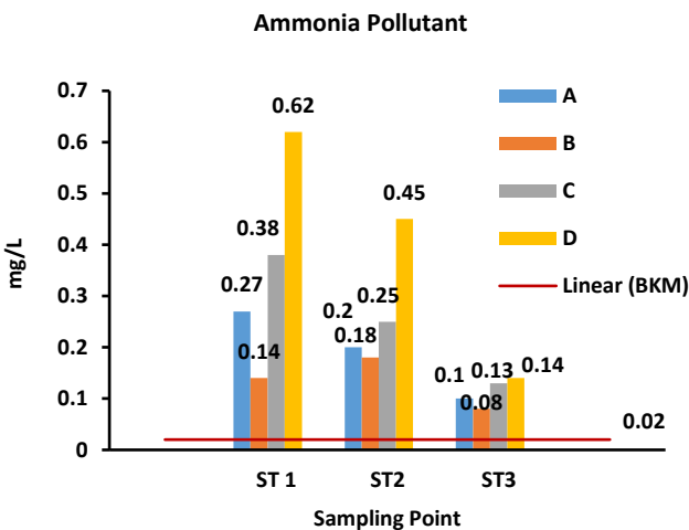
Figure 2. Ammonia pollutants in Keduang watershed from agricultural
