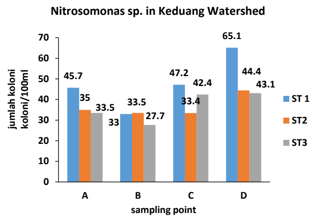
Figure 4. Nitrosomonas sp. in wastewater and river water
