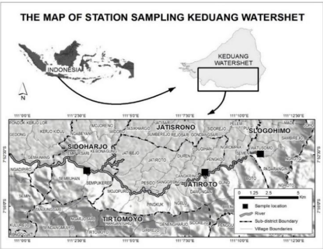
Figure 1. The map of station sampling Keduang watershed
