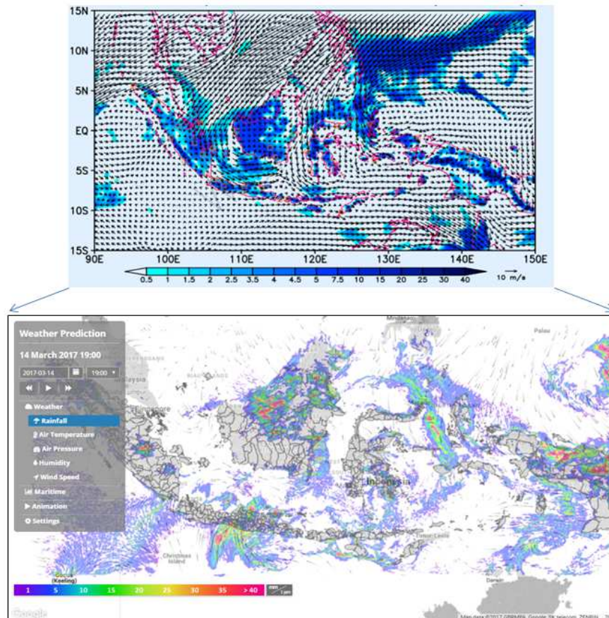
Figure 3 Upgrading weather prediction resolution to 5 km.
