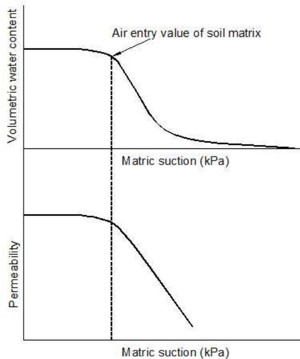
Figure 2 Schematic of SWCC and permeability function of cracked soil considering the cracked soil as a material with a unimodal pore size distribution.
