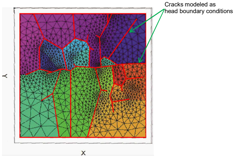
Figure 7 Example of plan view of a 3-D numerical model of a cracked soil specimen after 33 minutes of lateral flow.
