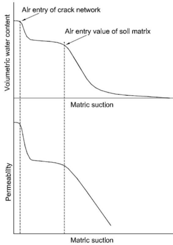
Figure 4 Schematic of the SWCC and permeability function of cracked soil considering the cracked soil as a material with a bimodal pore size distribution.
