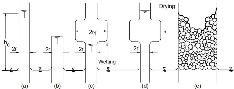
Figure 3 Capillary rise in soil (redrawn from Taylor, [23]).
