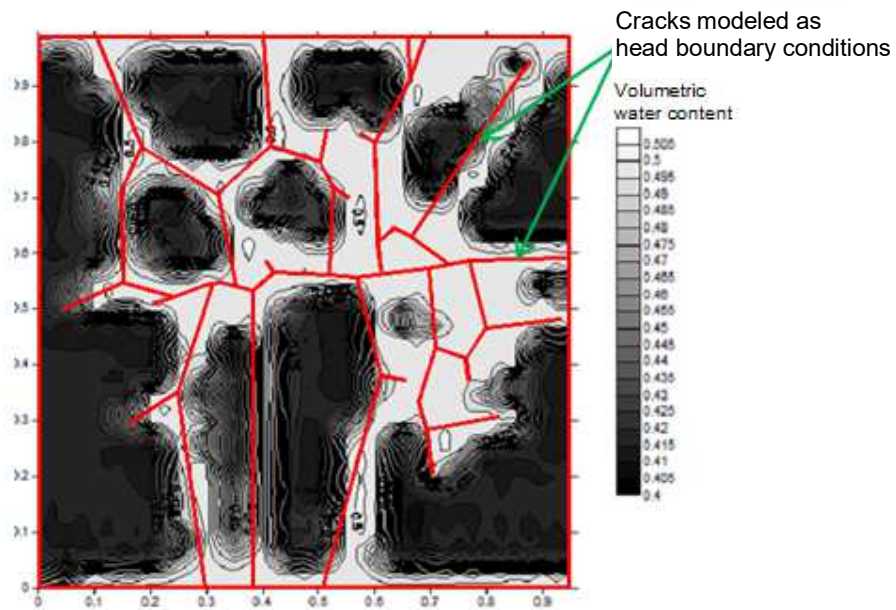
Figure 8 Example of a contour of water content in the numerical model of a cracked soil specimen after 33 minutes of lateral flow.
