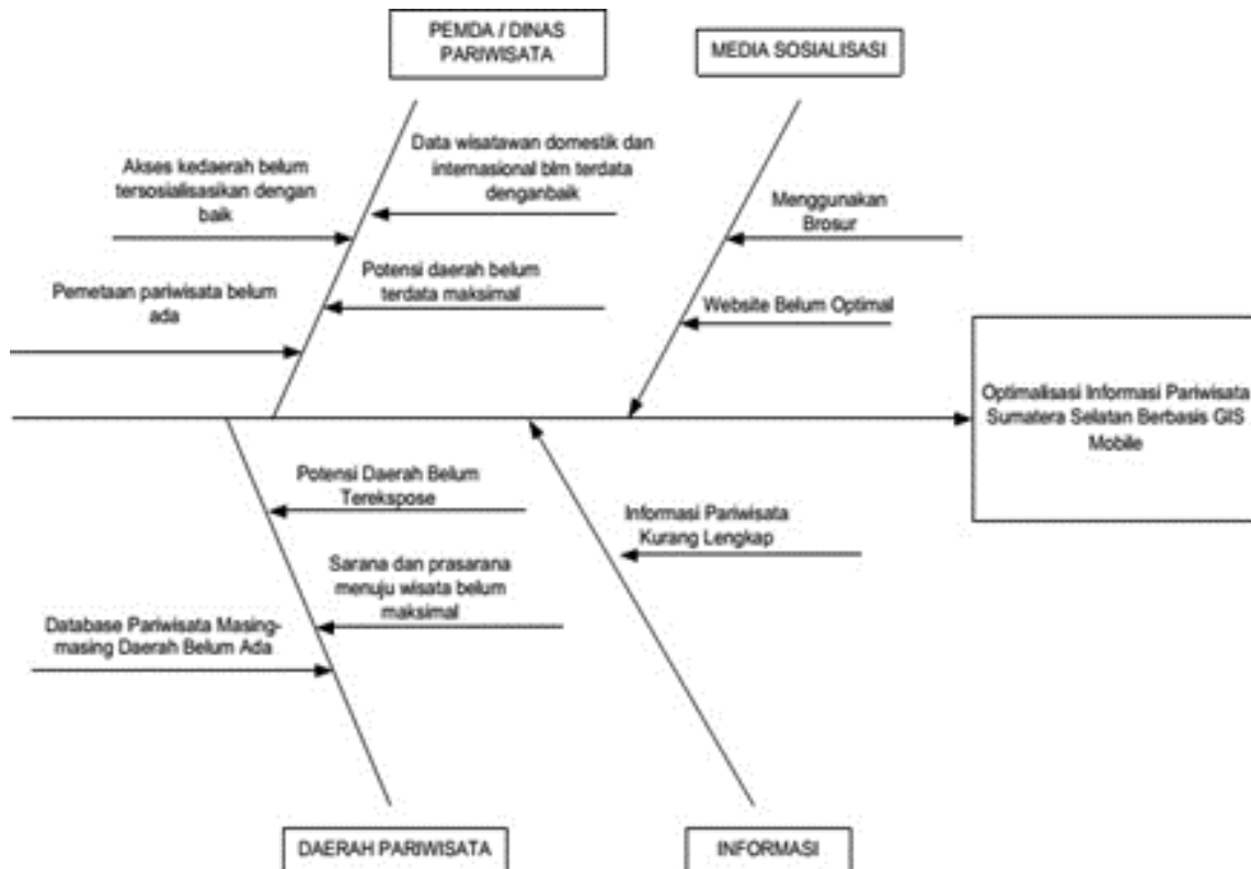
Gambar 1 Diagram Fishbone
