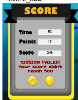
Gambar 14. Rule 7
