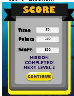
Gambar 13. Rule 6
