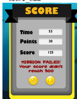
Gambar 11. Rule 4
