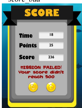
Gambar 8. Rule 1
