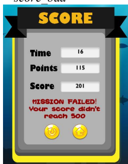
Gambar 9. Rule 2
