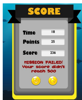
Gambar 7. Score Gagal
