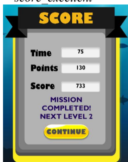
Gambar 15. Rule 8
