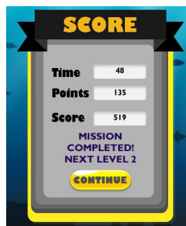
Gambar 6. Score Lolos
