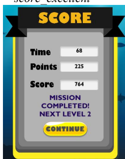
Gambar 16. Rule 9
