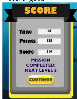
Gambar 12. Rule 5
