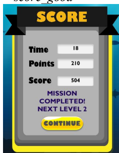
Gambar 10. Rule 3
