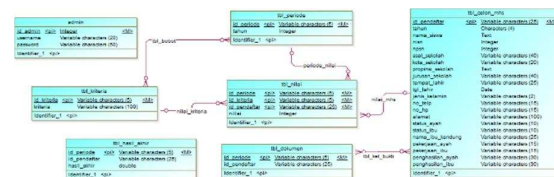
Gambar 4. Conceptual Data Model
