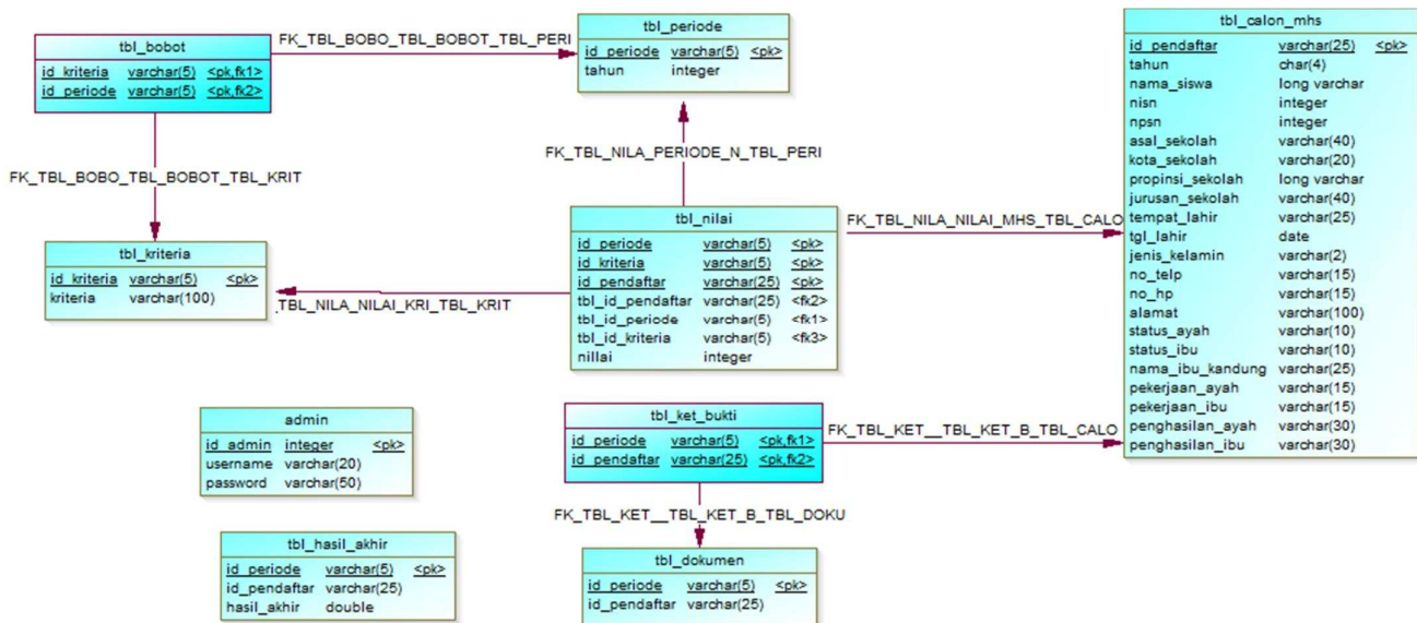
Gambar 5. Physical Data Model
