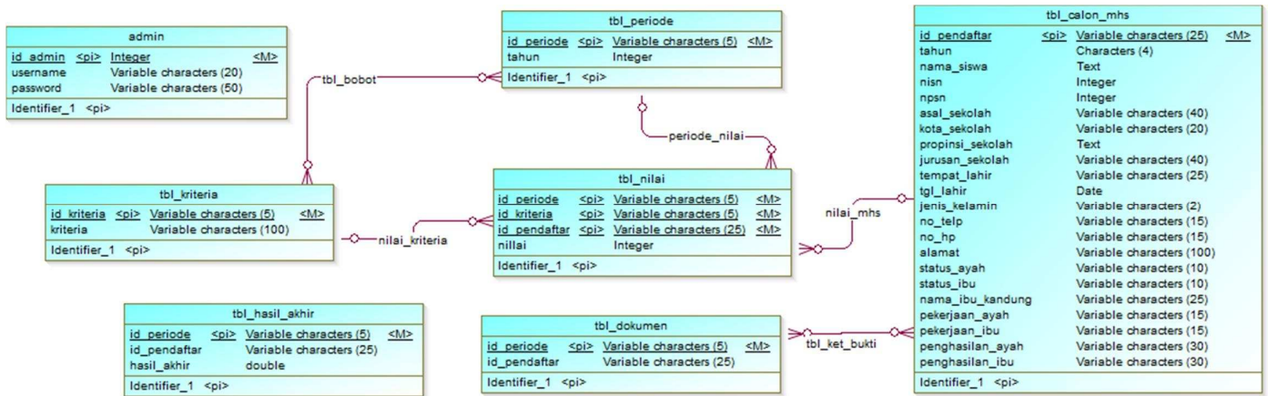
Gambar 4. Conceptual Data Model
