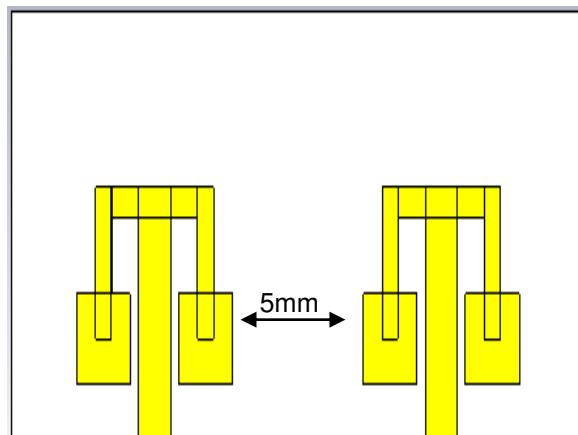
Figure 2. Two elements of an antenna
