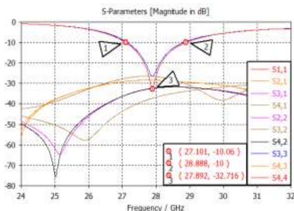
Figure 9. Simulated S-parameters of four elements of the antenna
