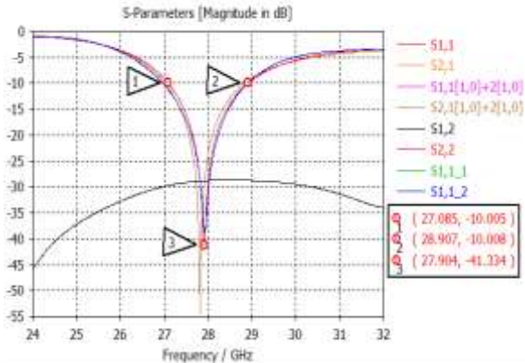
Figure 7. The reflection coefficient of two elements MIMO antenna
