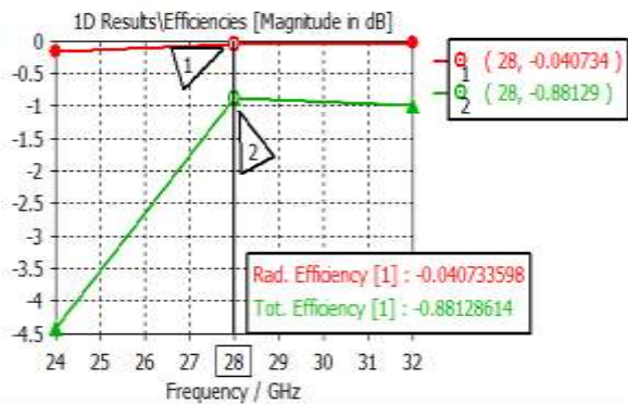
Figure 6. Radiation efficiency and total efficiency of the single element
