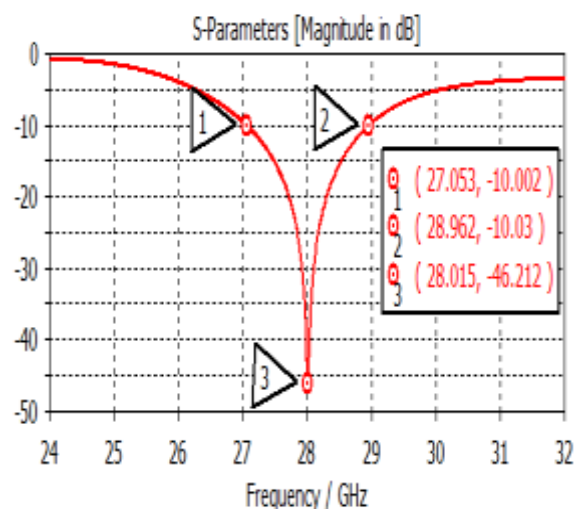
Figure 4. The simulated reflection coefficient of a single element
