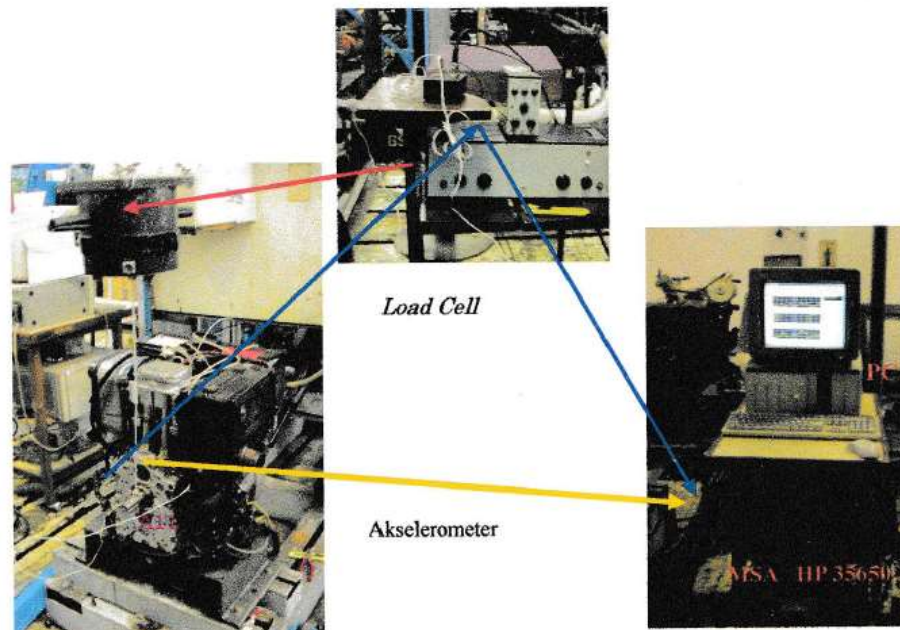
Figure 4. Photo of Set-up testing frequency response function
