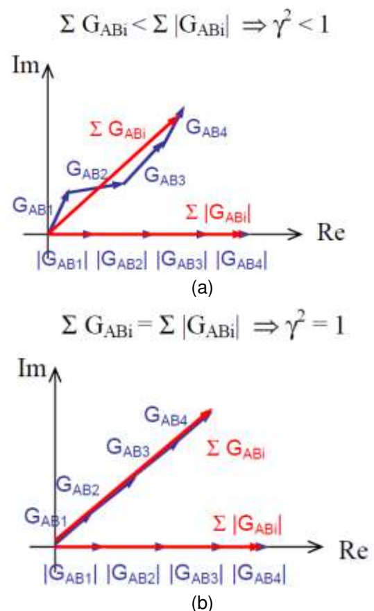
Figure 2. Effect of Noise on coherence: (a) with Noise and (b) without Noise
