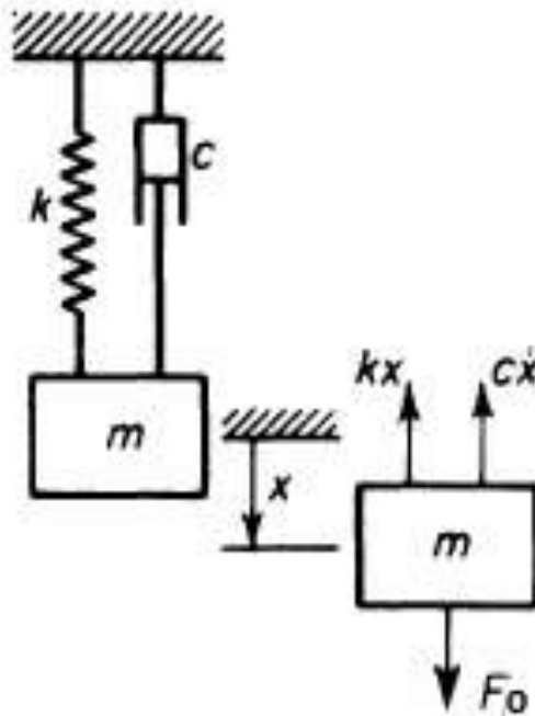
Figure 1. SDOF Vibration System Model
