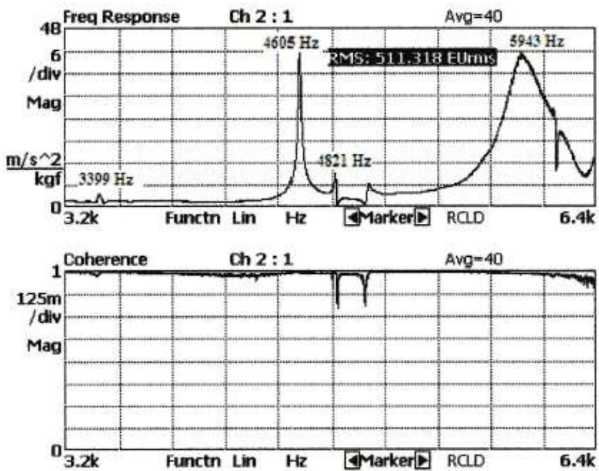
Figure 7. The result of FRF Point measurement of the frequency range from 3200 - 6400 Hz
