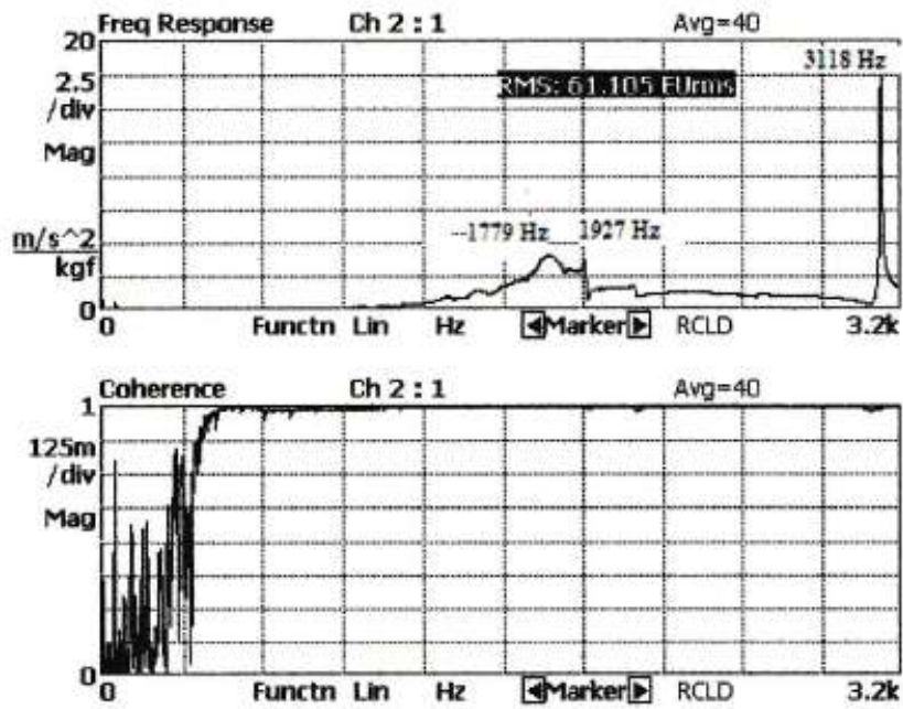
Figure 6. The Result of FRF Point measurement for frequencies range (0 - 3200 Hz)
