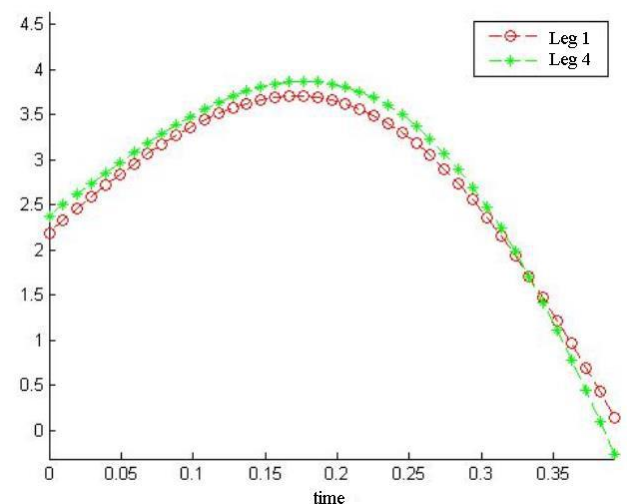
Fig. 7: Soil reaction forces on legs 1 and 4
