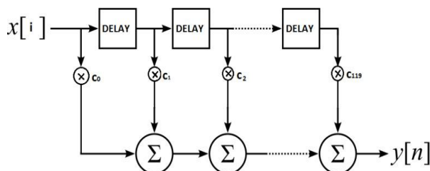
Fig.1. FIR Filter
