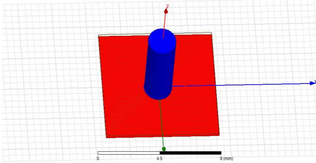
Fig. 1 Microstrip circular patch antenna without shorting pin
