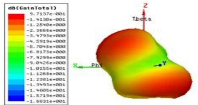
Fig. 5 3D Polar Plot (without shorting pin)
