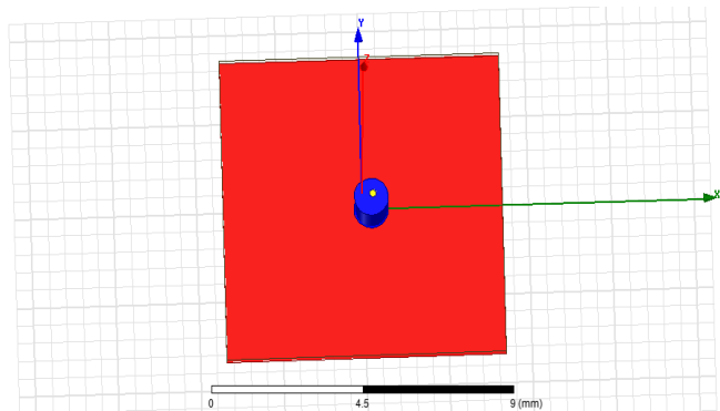
Fig. 2 Microstrip circular patch antenna with shorting pin
