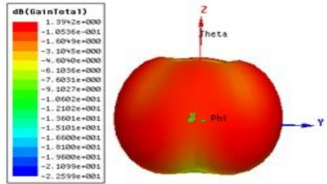
Fig. 4 3D Polar Plot (with shorting pin)
