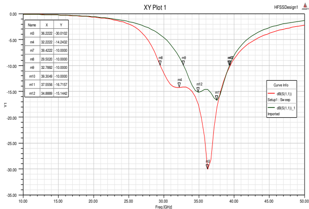
Fig. 3 Return loss (--- with shorting pin --- without shorting pin)
