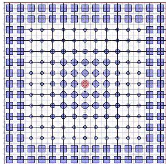
Fig.1 Inner two layer d=0.12\mu\text{m} , 3 rd layer d=0.9\mu\text{m} , 4 th and 5 th layer d=0.6\mu\text{m} . 6 th and 7 th layer W=L=1.2\mu\text{m} . pitch ( \Lambda ) = 2.0\mu\text{m} .
