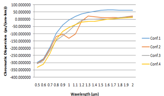
Fig.2 Simulation results graph of square lattice PCF of borosilicate crown glass (BK7).
