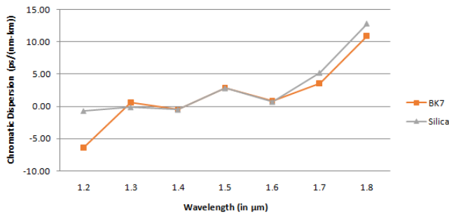
Fig.5 Dispersion graph of proposed PCF with Borosilicate and Silica at 1.2 to 1.8μm wavelength.
