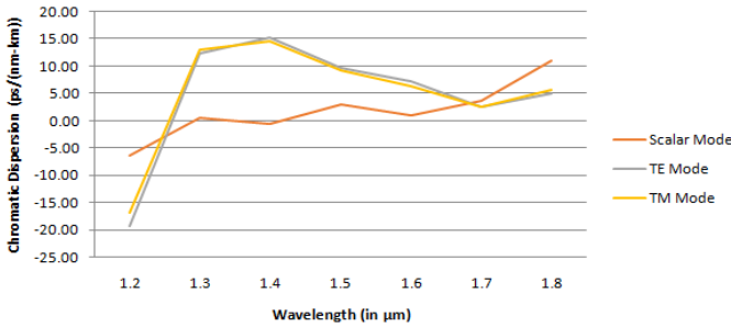
Fig.4 Dispersion graph of proposed PCF of BK7 in Scalar, TE and TM mode at 1.2 to 1.8μm wavelength.
