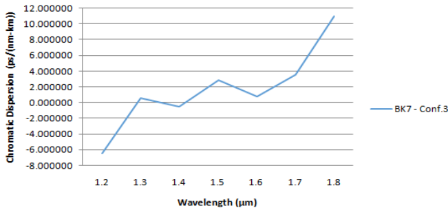
Fig.3 Near zero ultra flattened dispersion graph of proposed PCF of BK7 at 1.2 to 1.8μm wavelength.
