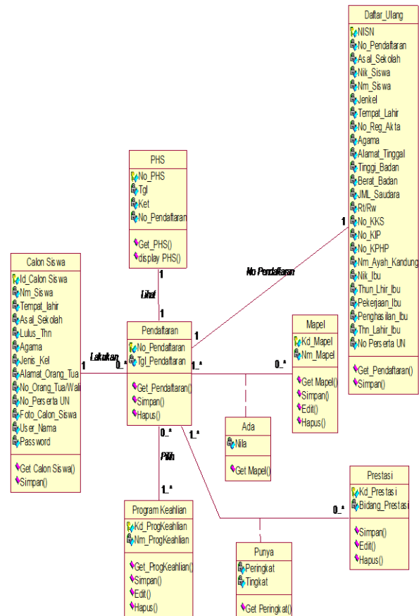
Gambar 11. Class Diagram
