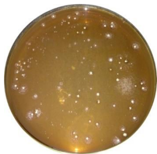
Figure 2. Actinomycetes isolates growth in HV agar media
