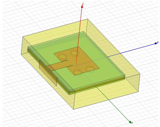
Figure- 1.3 MS Antenna with EBG Structure ( 4 air cavities of radius r = 4 mm)
