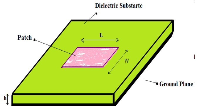
Figure- 1.1 Geometry of Microstrip Patch Antenna
