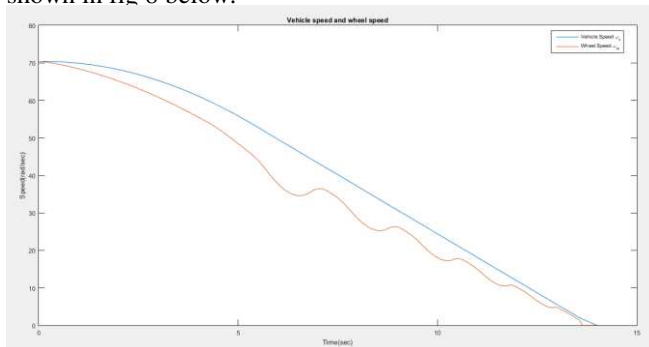
Fig 8: Vehicle speed and wheel speed behavior
