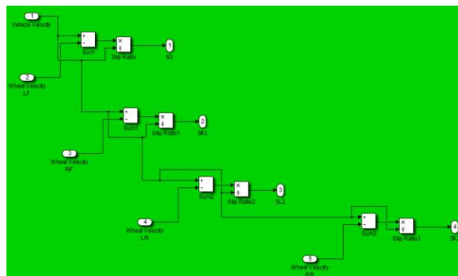
Fig 4: simple ABS controller model for slip ratio calculation
