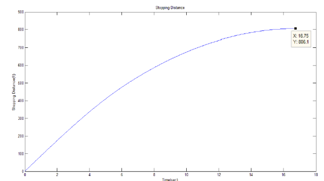
Fig 11: Stopping distance without ABS
