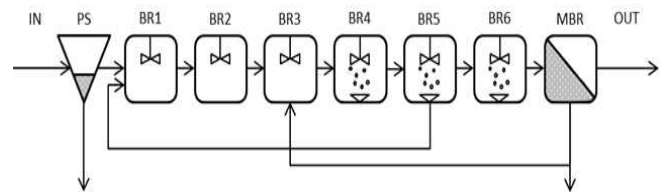
Figure 1. Schematic overview of the treatment line at HammarbySjöstadswerk used for development of the soft sensors. The incoming water is named IN and effluent is named OUT. The line consists of a pre-sedimentation (PS), three unaerated bioreactors (BR1-3), three aerated BR (BR4-6) and a membrane bioreactor (MBR) with the submerged UF
