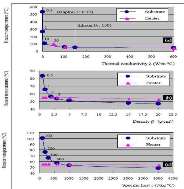
Fig. 11 Effects of substrate and heater's material properties to the sensor sensitivity at the dimensional condition of 400- \mu\text{m} thick substrate and 5- \mu\text{m} thick heater with 1- \mu\text{m} thick \text{SiO}_2 layer. Input power is 50mW and input power during time is 1ms: (a) effect of thermal conductivity; (b) effect of density; and (c) effect of specific heat.
