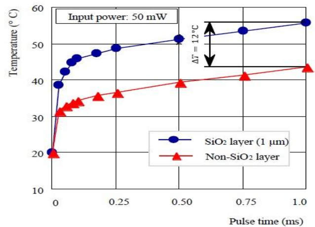
Fig. 6 Silicon dioxide layer effect to the thermal isolation
