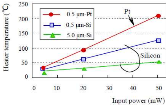
Fig. 9 Heater size and material effect ( \tau=1 ms)
