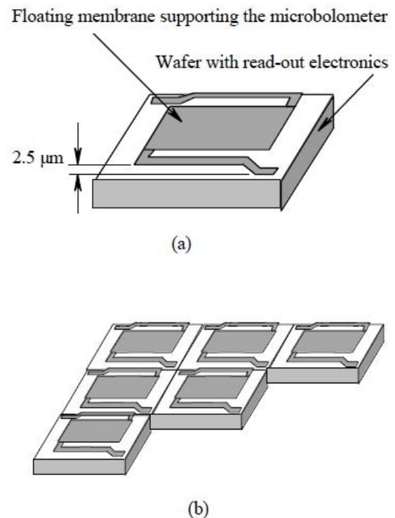
Fig. 3 Element structure of a matrix thermal sensor array by surface micromachining. This structure was developed at Honeywell, USA and applied for designing uncooled focal plane arrays [29]: (a) Single element, and (b) Arrayed elements image.
