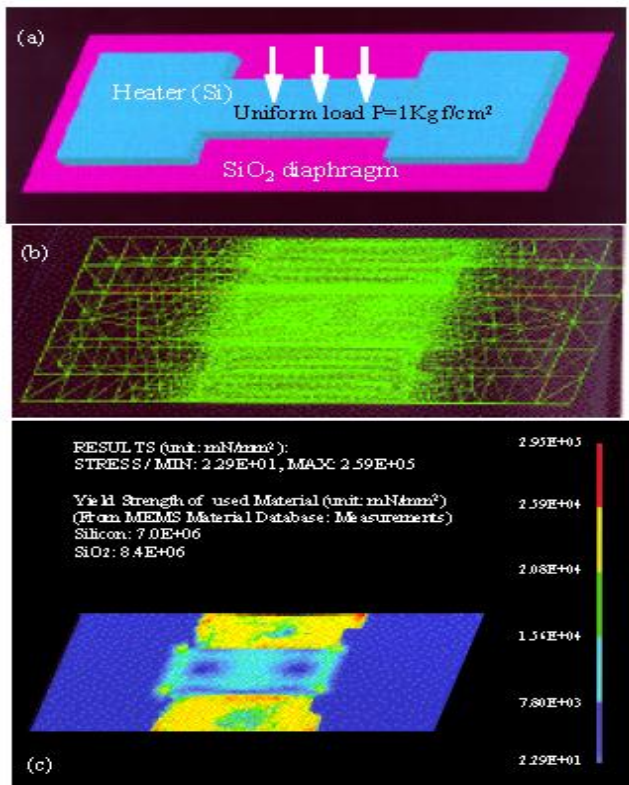
Fig. 12 Mechanical strength analysis by I-DEAS: (a) simulation model; (b) meshed state for calculation, and (c) calculation results by simulation.
