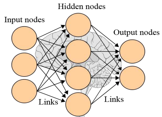
Figure 2.4.Neural network
