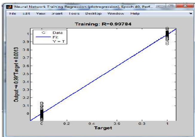
Figure 3.1 Regression
