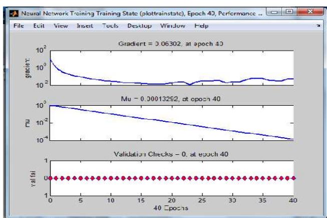
Figure 3.3 Training State
