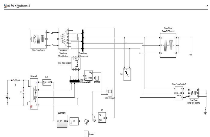
Figure 5.5: Model for Line-Line-Ground fault condition
