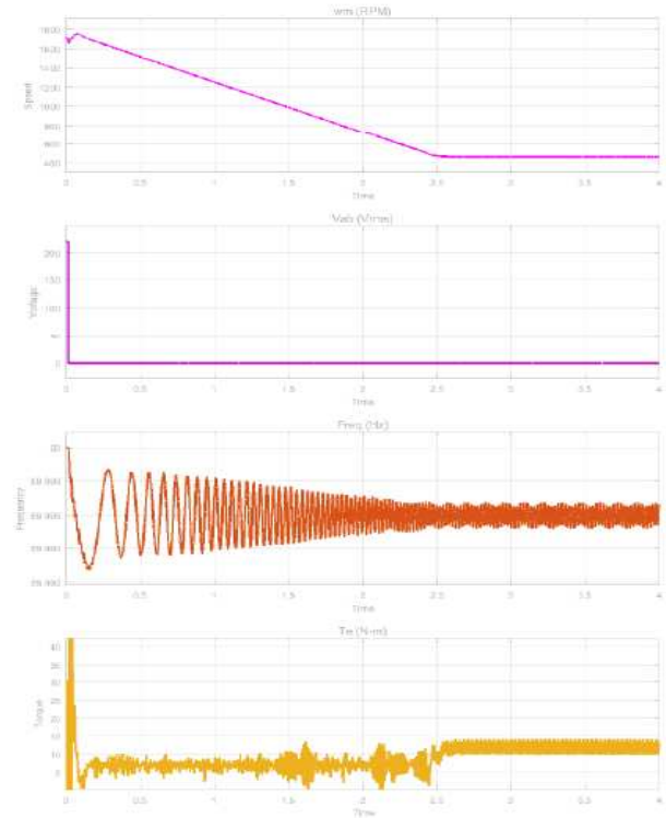
Figure 26 Increase in load torque (8 N-m to 11.9 N-m)
