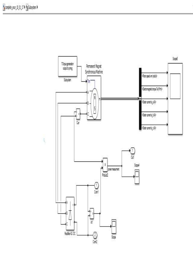
Figure 5 Wind Model
