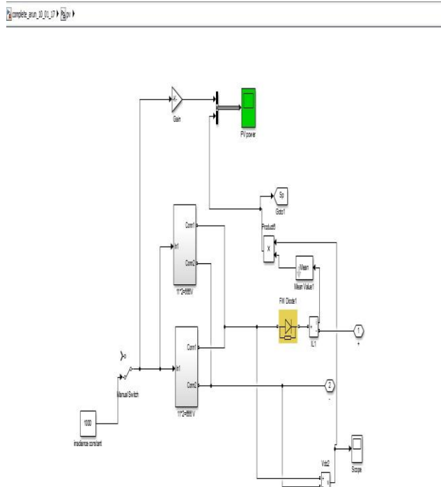
Figure 4 PV Array Model
