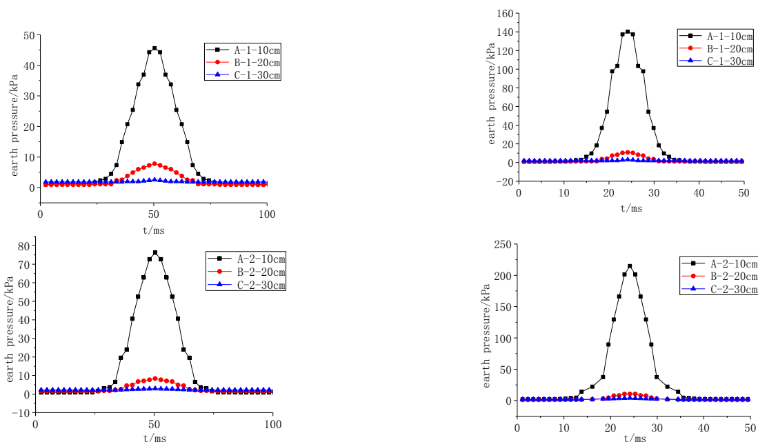
Figure 7. Curves of earth pressure with time in 7.5N·m tamping energy
