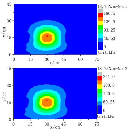
Figure 13. Influence range at the depth of 10cm by 18.75N·m tamping energy
