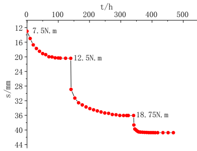
Figure 6. Curves of settlement with time at the top of soft soil under dynamic consolidation
