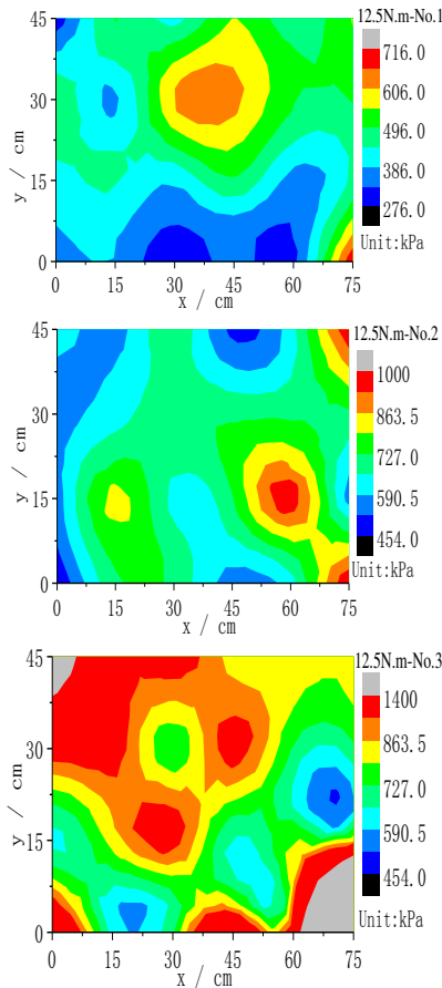
Figure 4. the soil body resistance nephogram when ramming energy is 12.5N·m
