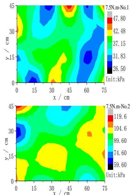
Figure 3. the soil body resistance nephogram when ramming energy is 7.5N·m
