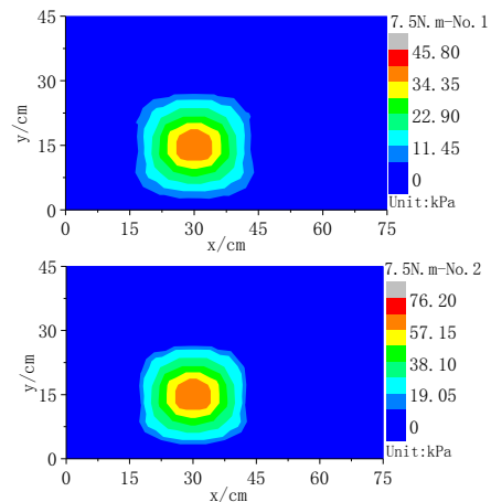
Figure 11. Influence range at the depth of 10cm by 7.5N·m tamping energy
