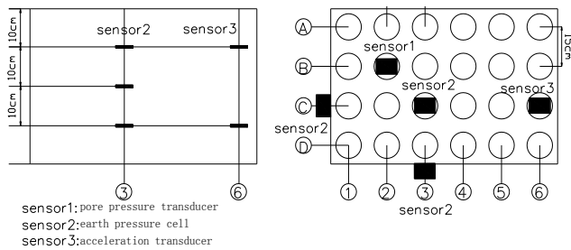
Figure 2. Sketch map of sensor section and plane layout of tamping point
