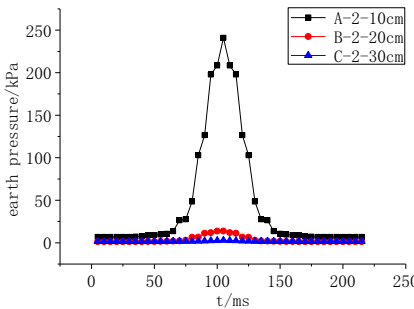
Figure9. Curves of earth pressure with time in 18.75N·m tamping energy
