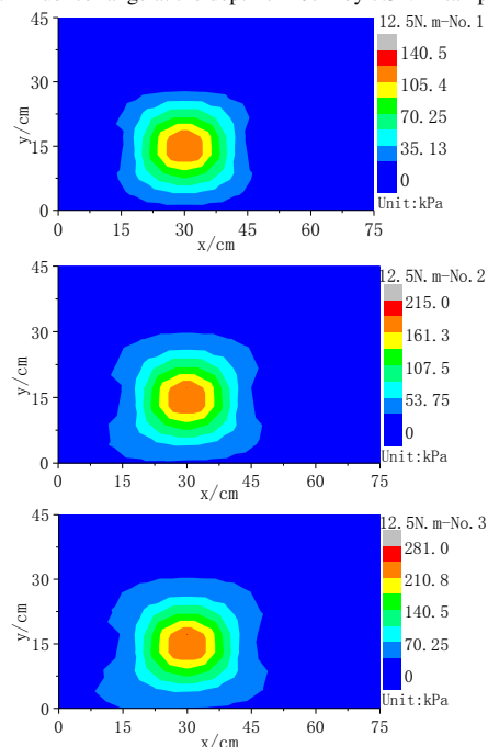
Figure 12. Influence range at the depth of 10cm by 12.5N·m tamping energy
