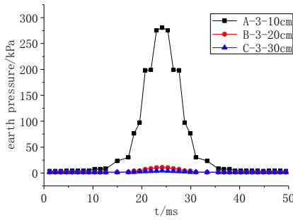
Figure8. Curves of earth pressure with time in 12.5N·m tamping energy
