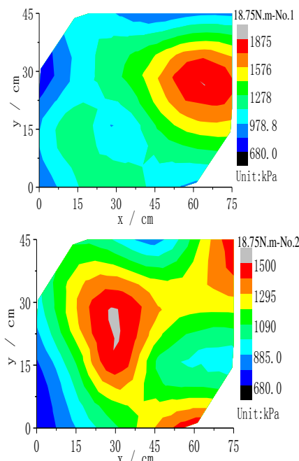
Figure 5. the soil body resistance nephogram when ramming energy is 18.75N·m
