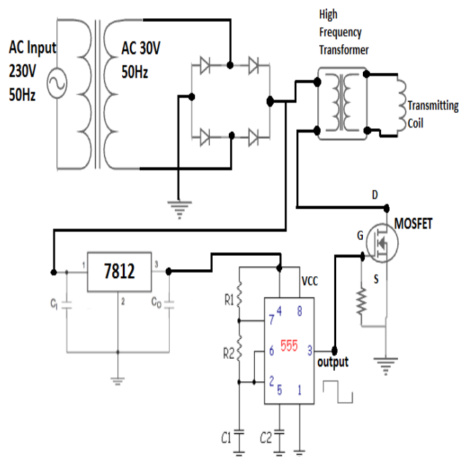
Fig.2. Transmitter Section
