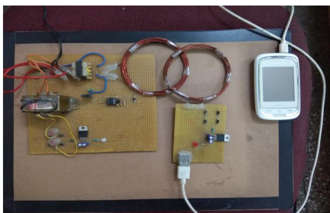
Fig.4. Experimental Setup
