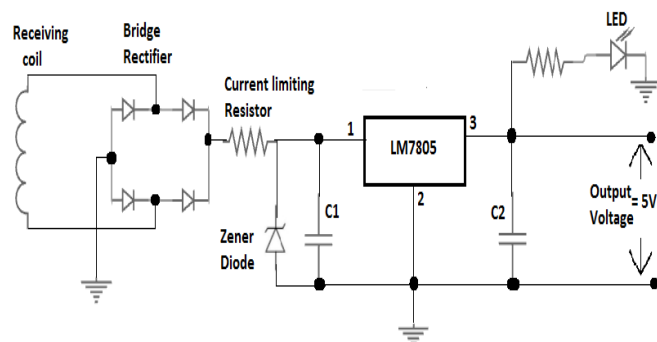
Fig.3. Receiver Section
