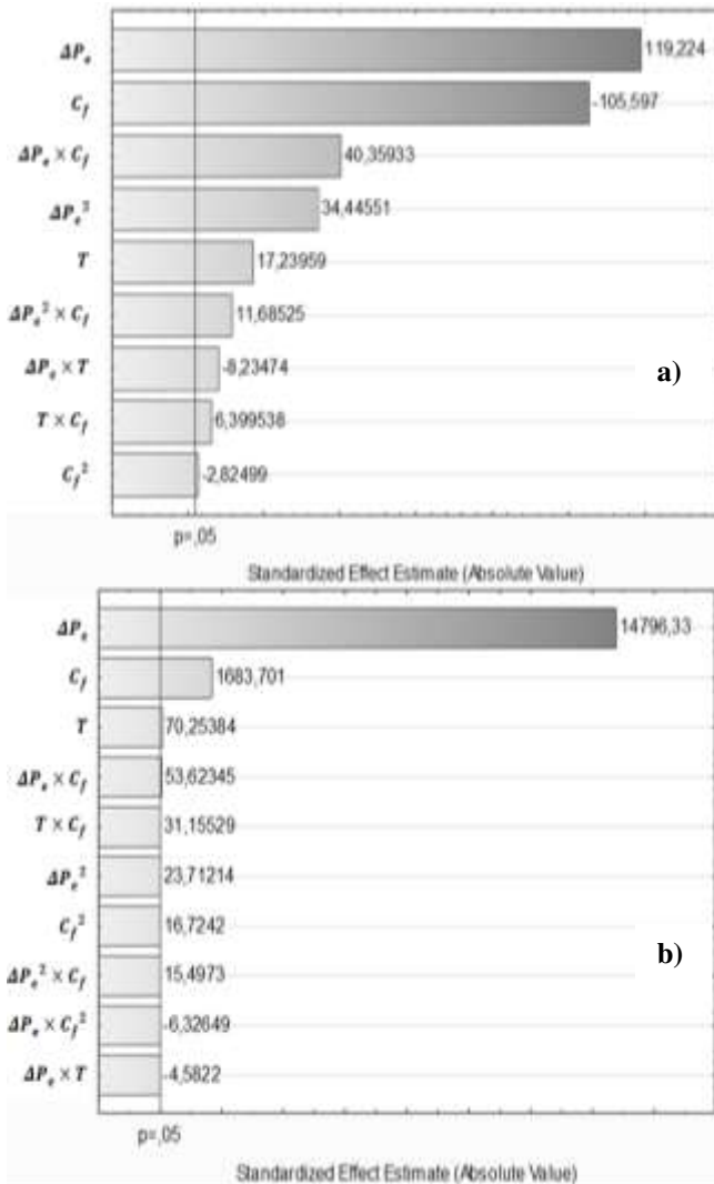
Fig. 3. Pareto charts of effects for the responses: (a) rejection and (b) SEC.
