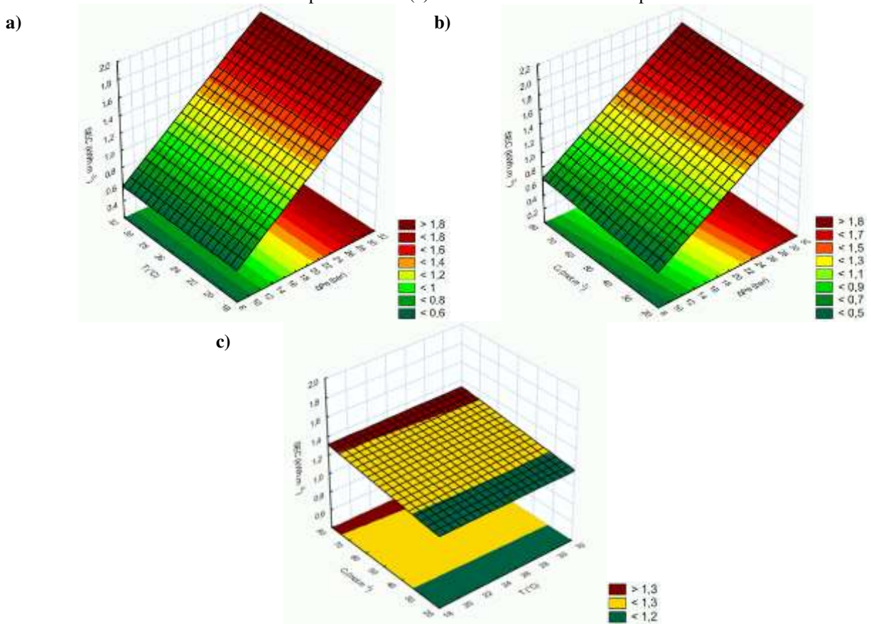
Fig. 5. Response surfaces of SEC as a function of: (a) temperature and effective pressure; (b) feed concentration and effective pressure and (c) feed concentration and temperature.
