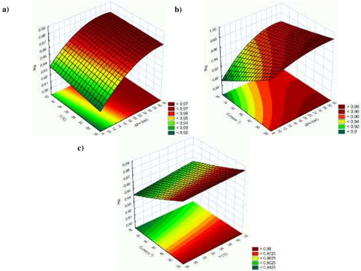
Fig. 4. Response surfaces of rejection as a function of: (a) temperature and effective pressure; (b) feed concentration and effective pressure and (c) feed concentration and temperature.
