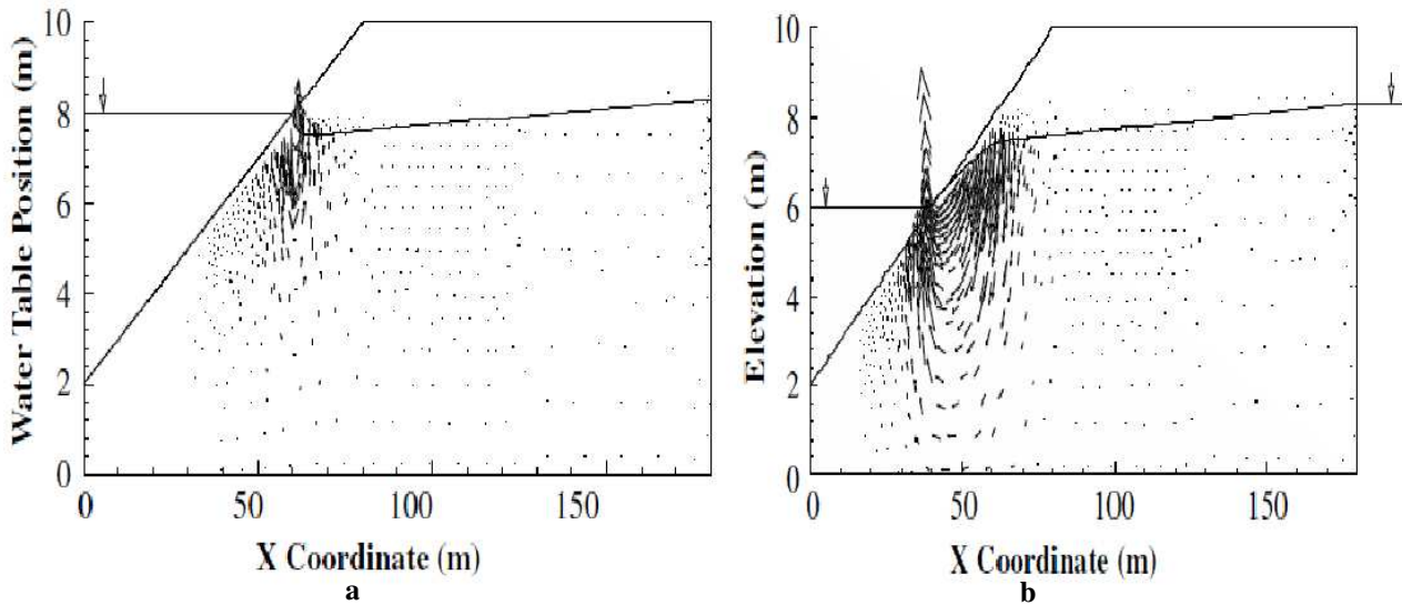
Fig 4: High and low water levels with velocity field distribution [24]
