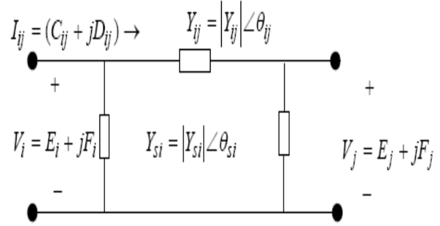
Figure 2: Transmission Line Model
