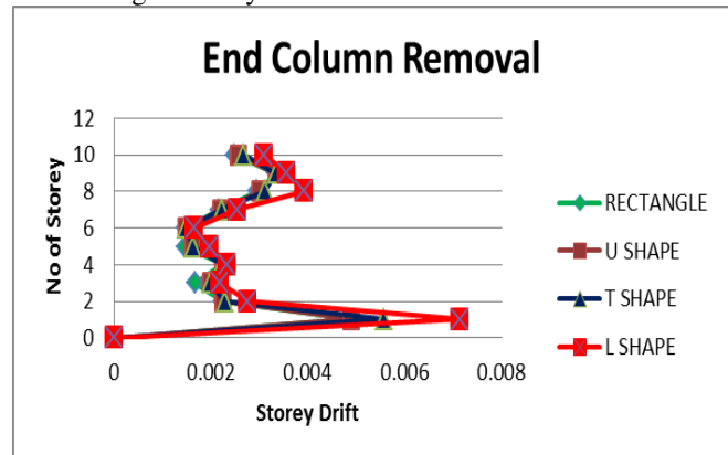
Fig. 3 Storey Drift for End Column Removal
