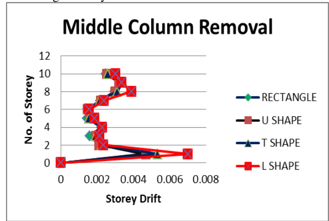
Fig 1 Storey Drift for Middle Column Removal
