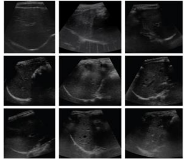
Figure 5 Experimental Dataset
