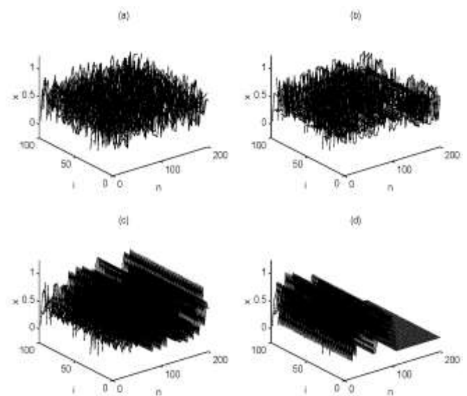
Fig.4. Spatiotemporal evolution of the coupled map lattice, with (a) \epsilon = 0.25 (b) \epsilon = 0.45 (c) \epsilon = 0.55 (d) \epsilon = 0.75
