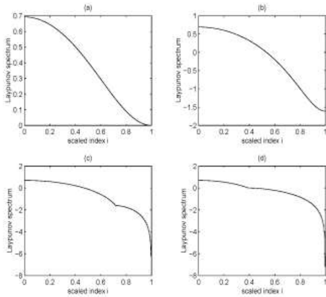
Fig.1. Scaled Lyapunov spectra for coupled map lattices, with (a) \epsilon = 0.25 (b) \epsilon = 0.45 (c) \epsilon = 0.55 (d) \epsilon = 0.75
