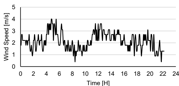
Figure 4. Wind speed
