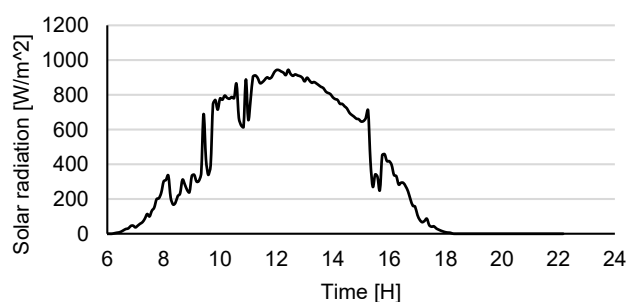
Figure 3. Solar radiation
