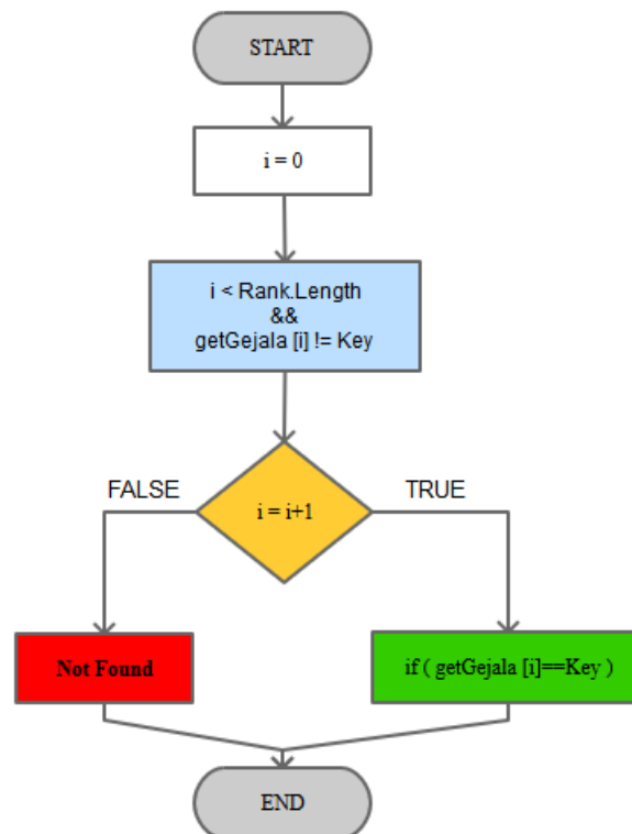
Gambar 3 Flowchart Sequential Search
